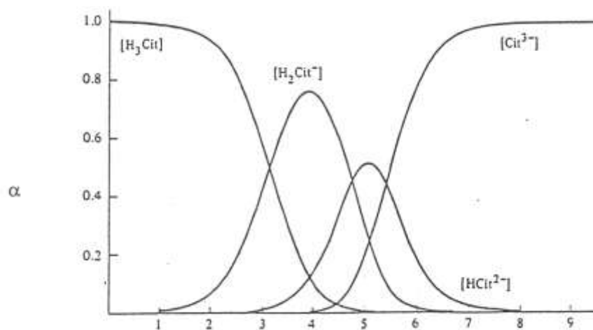
Citric Acid ( pK_a values of 3.13, 4.76, and 5.41)
