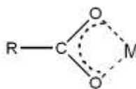
Chelate Bonding
