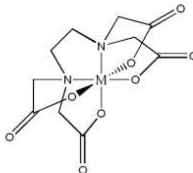
Chelate bonding to a metal
