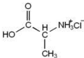
alanine hydrochloride
