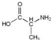
alanine
