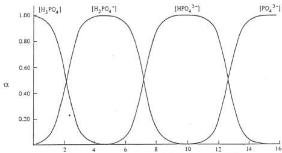
Phosphoric Acid ( pK_a values of 2.12, 7.21, and 12.66)
