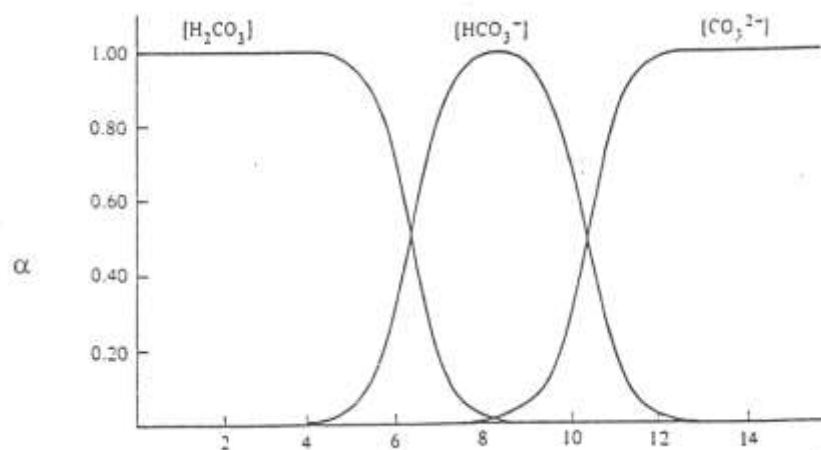
Carbonic Acid ( pK_a values of 6.4 and 10.4)
