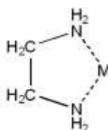
Chelate Bonding
